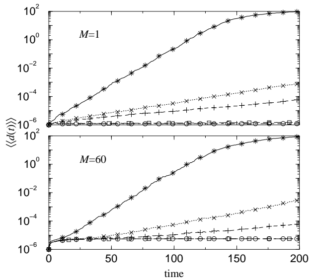
FIG. 1. Average distance in phase space between pairs of trajectories corresponding to initial conditions such that d(0) \leq 10^{-6} and \epsilon = 0.01 (circle), 0.1 (square), 1 (plus), 2 (cross), and 10 (asterisk) for M = 1 and M = 60 with N = 300,000 . Time is measured in natural units.
