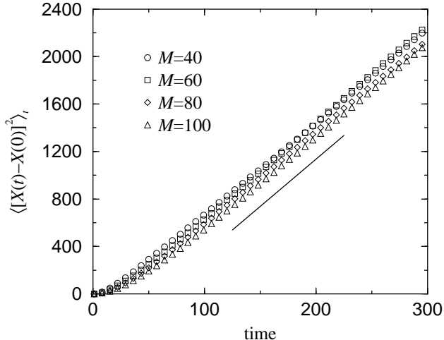
FIG. 2. Mean-square displacement of the impurity for \epsilon = 10 . The solid line, with slope 2D = 7.95 , has been added for reference.
