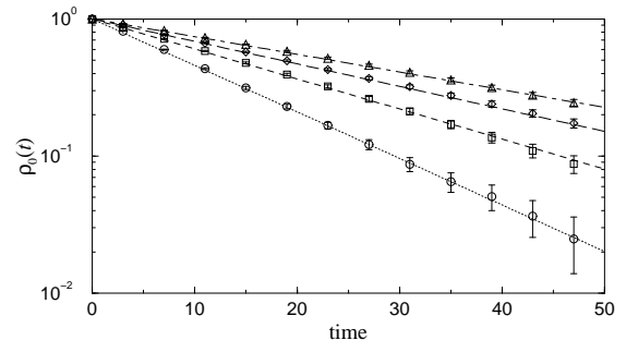
FIG. 4. Logarithm of the MACF of the impurity for \epsilon = 10 . Symbols have the same meaning as in Fig. 2. The straight lines for each value of M correspond to the fit \exp(-t/\tau) .
